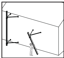
1 Install wood pole to work wall
