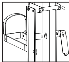
2 Install Steel Pump Jack to Wood pole
