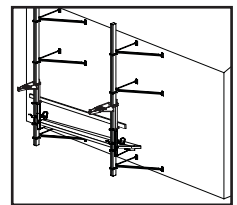
5 Install walk platform
